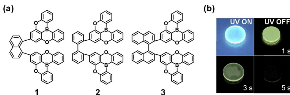
Figure 1. (a) Chemical structures of 1-3 and (b) photographs of the luminescence 1 in PMMA film under UV irradiation and after removal of the UV lamp at room temperature.
