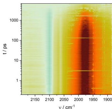
Figure 1. fsIR spectroscopy of [Ru(tpy)(bpy)(CN)Ru(py)_4(DMAP)]^{3+} under 480 nm excitation, in acetonitrile at room temperature. The broad, intense and down-shifted C\equiv N stretching signal indicates a Class III behavior.
