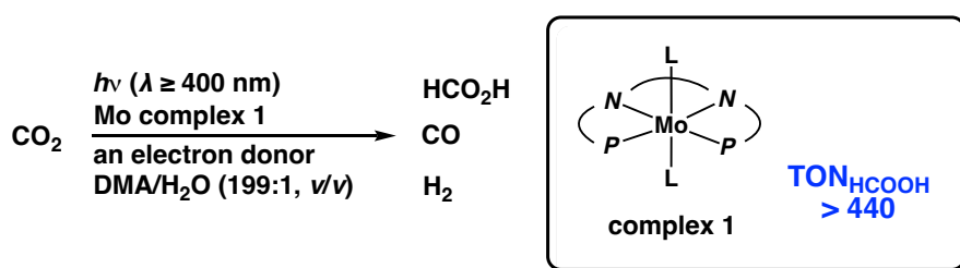
Scheme 1. Photocatalytic reduction of CO 2 with a Mo complex as a photocatalyst under visible light irradiation ( \lambda \geq 400 nm)
