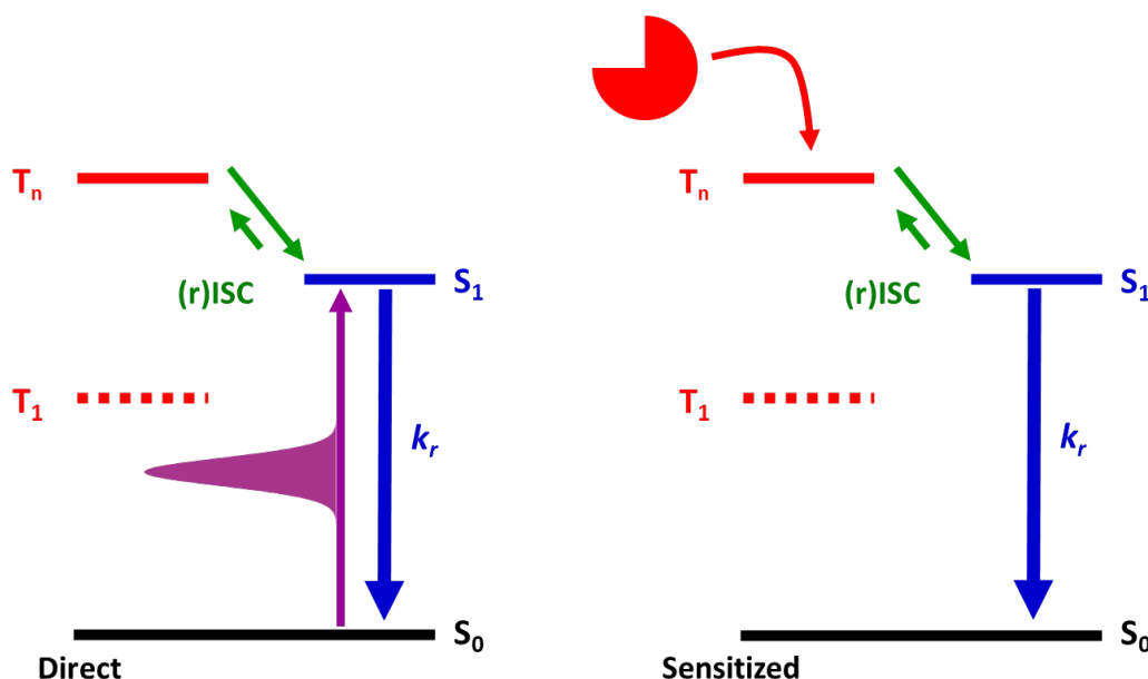
Figure 1. Investigation of HIGHrISC behavior via direct (left) and sensitized (right) excitation. In the direct excitation experiment, the chromophore is promoted to the S_1 state by a laser pulse. Provided that the T_n state is in energetic reach, the equilibration of the two states can be monitored by time resolved spectroscopy. A suitable molecular sensitizer transfers population to the T_n state which is ensued by rISC and fluorescence emission.
