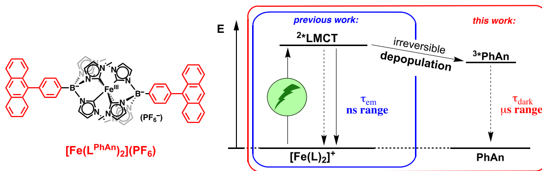
Figure 1. Structure of the investigated molecular dyad (left) and energy scheme comparing the established iron-based complex [4] with an emissive ligand-to-metal charge transfer ( 2^*LMCT ) excited state (blue box) and the newly designed dyad with an energy acceptor (PhAn) attached (red box).
