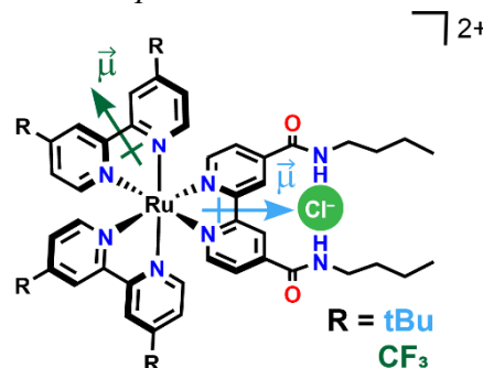
Figure 1. Metal-to-ligand charge transfer (MLCT) excitation results in chloride migration/release when the excited state was localized on the halide associated ligand (R = tertiary butyl) and not when the excited state was localized on an ancillary ligand (R = CF 3 ).
