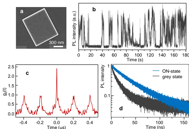
Figure 1. a) SEM image of a typical \text{CsPbBr}_3 perovskite quantum dot superlattice; b) Two-level blinking of a single superlattice; c) Second-order correlation function of PL from a single superlattice showing photon bunching; d) PL lifetime from ON and grey states of the blinking trace.
